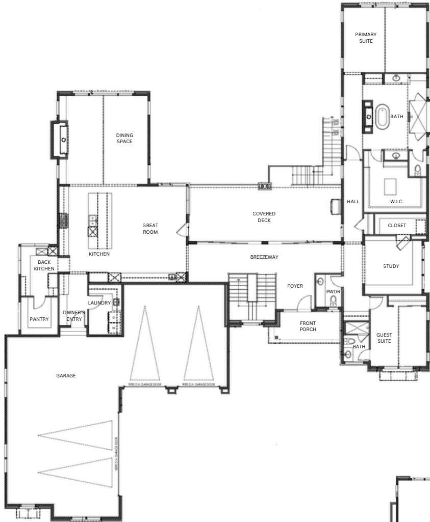
MAIN LEVEL // 3,261 SQFT FINISHED
