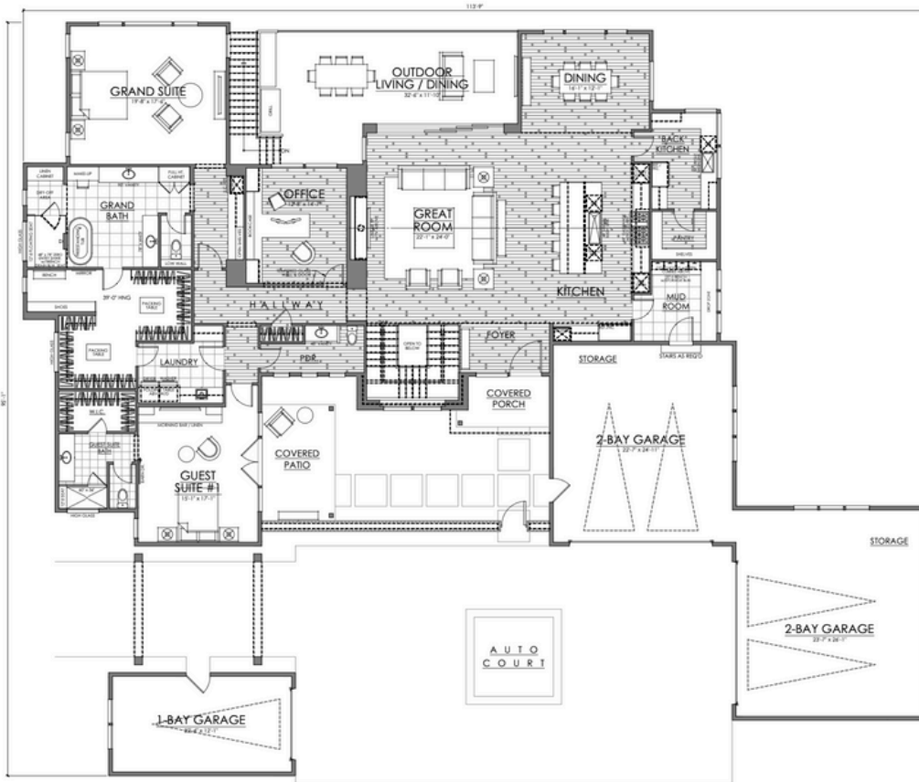
MAIN LEVEL // 3,491 SQFT TOTAL
