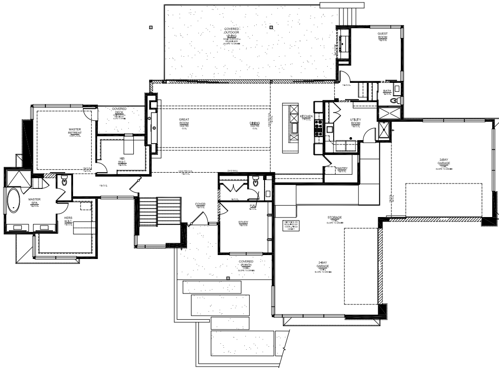
MAIN LEVEL // 2970 SQFT FINISHED
