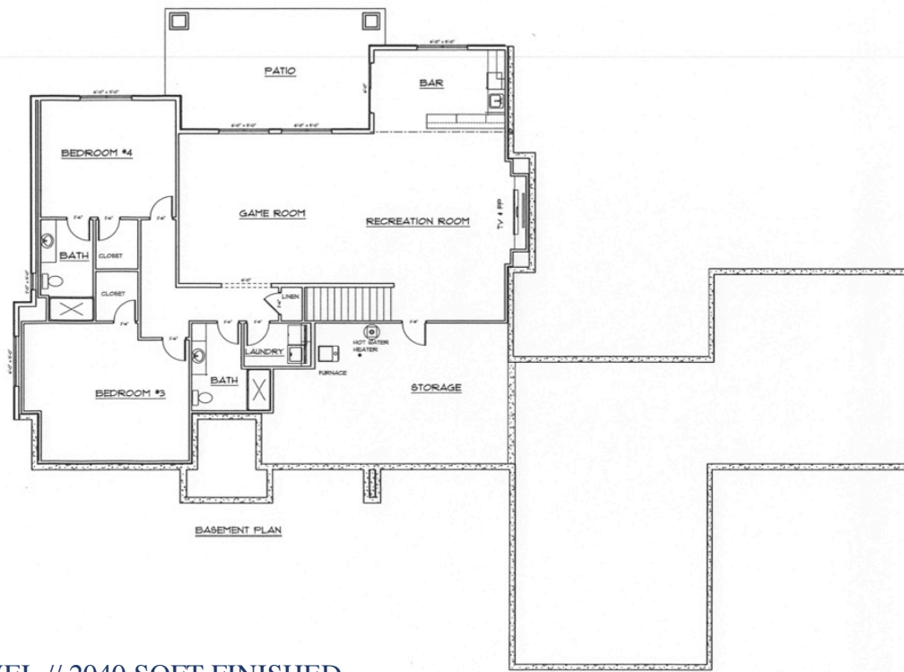
LOWER LEVEL // 2040 SQFT FINISHED
