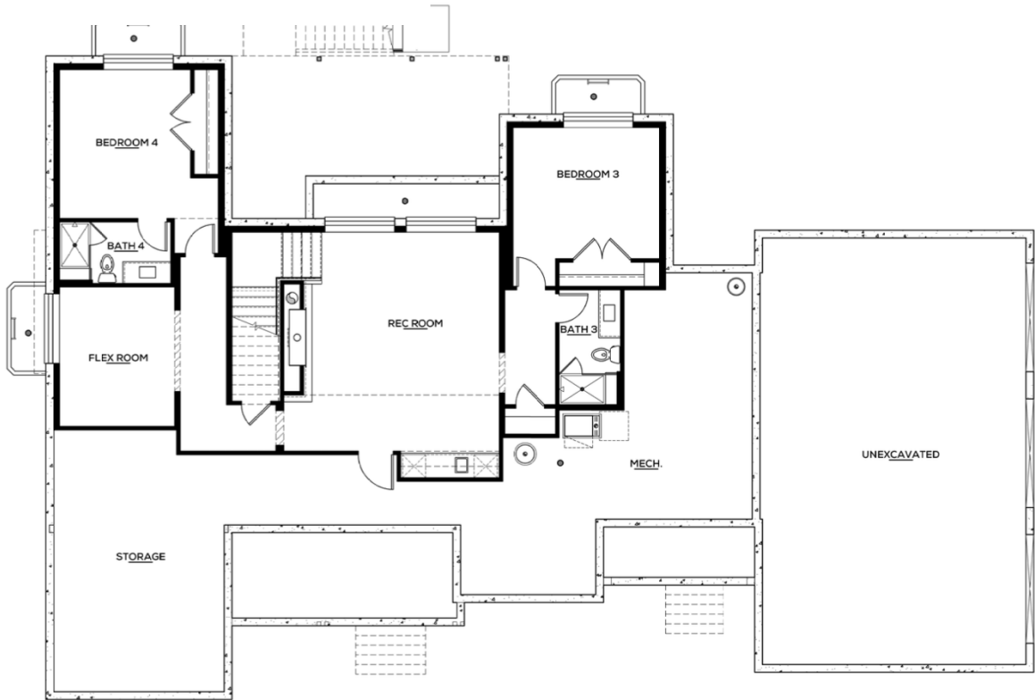
LOWER LEVEL // 1281 SQFT FINISHED
