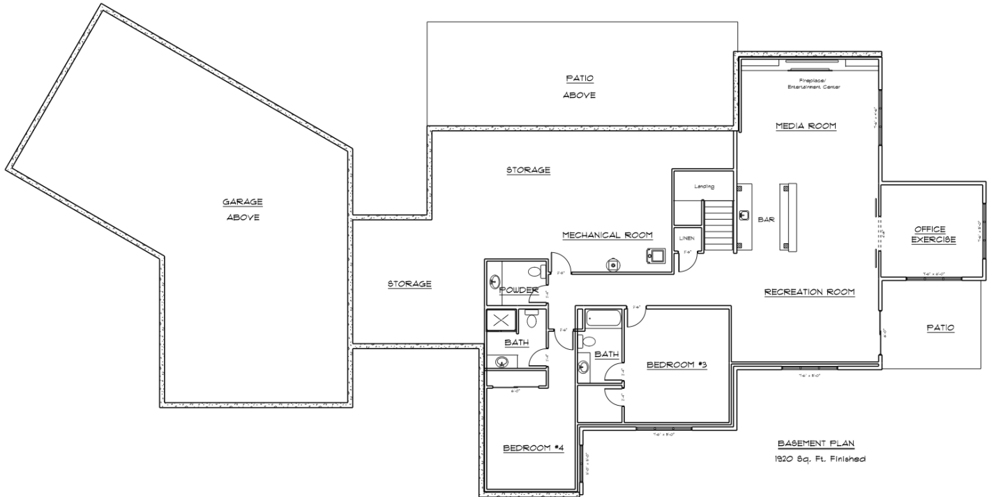
LOWER LEVEL // 1920 SQFT FINISHED
