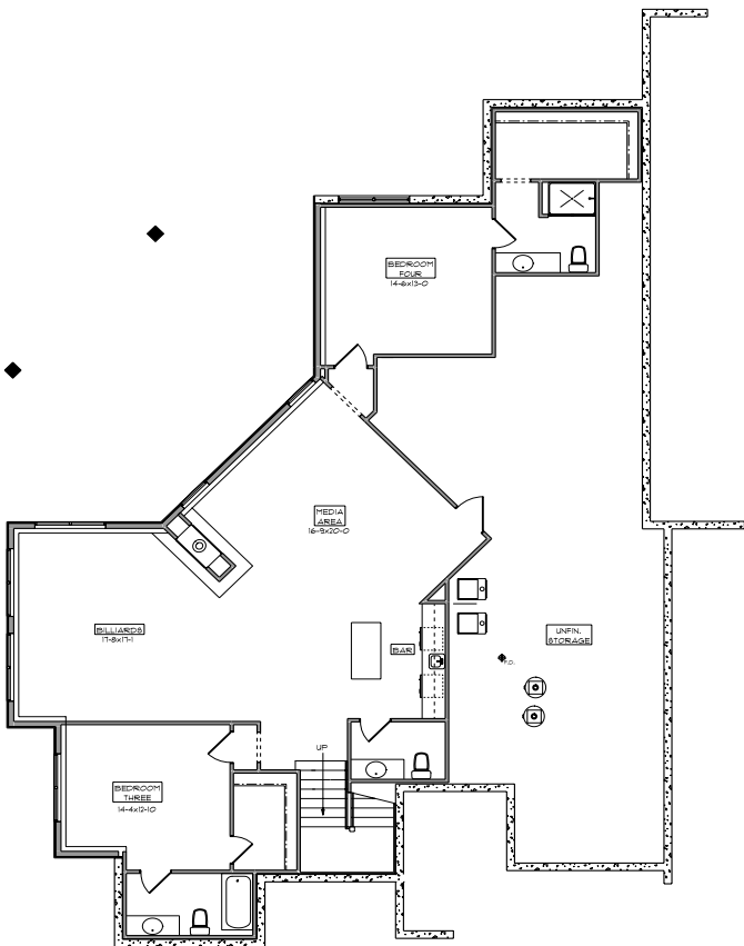
LOWER FLOOR PLAN 1,686 FinSqFt
