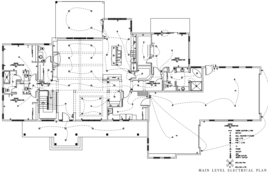
MAIN LEVEL // 2622 SQFT FINISHED
